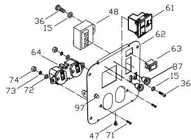
37 Control Panel Assembly IG2000/S1A-13100
